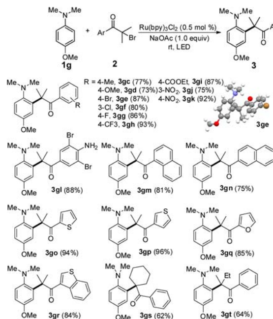
Scheme 3. Scope of \alpha -Bromo Ketones 2 a
