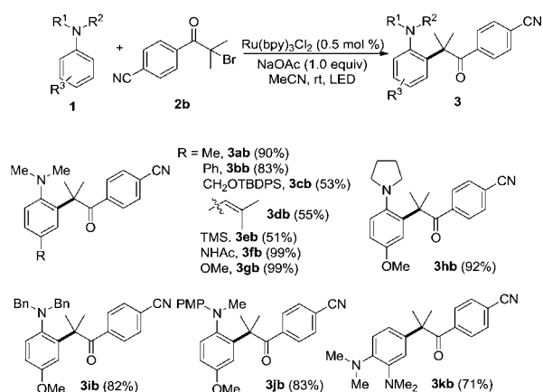
Scheme 2. Scope of Anilines 1 a
