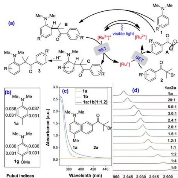
Scheme 5. Proposed Mechanism
