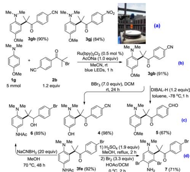
Scheme 4. Applications of Quaternary Alkylation
