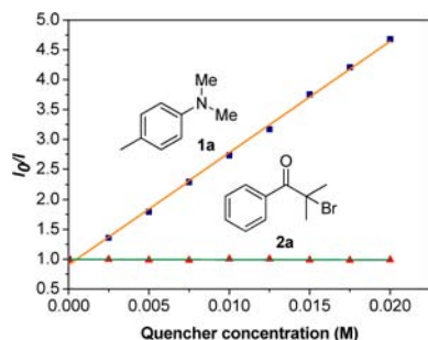
Figure 2. Fluorescent quenching of \text{Ru}(\text{bpy})_3\text{Cl}_2 .
